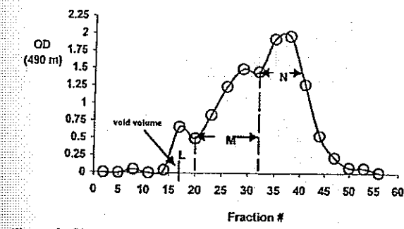
Figure 1. Size exclusion chromatography of fraction J on Sephacryl S-300.
