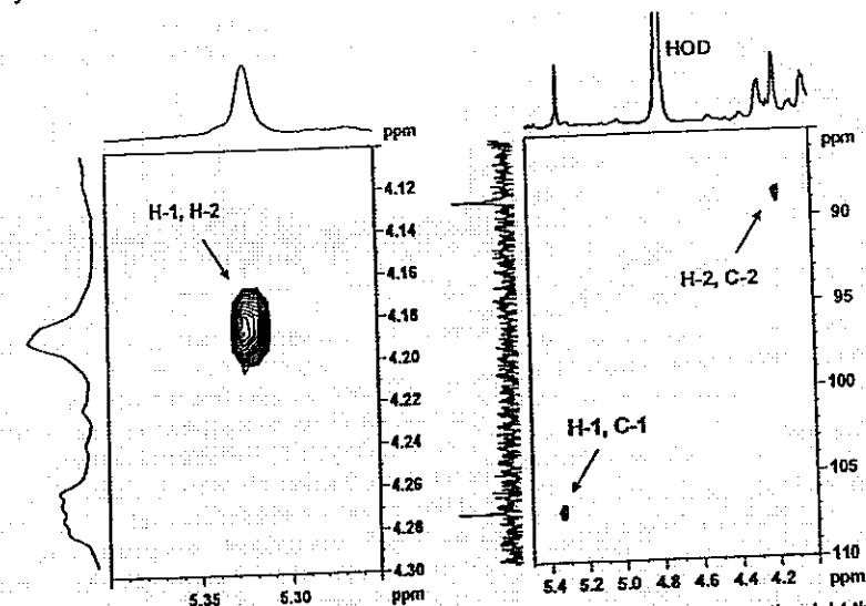
Figure 3. Portions of spectra of fraction R: on the left, the 500.1 MHz ^1\text{H} , ^1\text{H} DQF-COSY spectrum; on the right the ^1\text{H} , ^{13}\text{C} HSQC spectrum. The relevant correlations are annotated.
