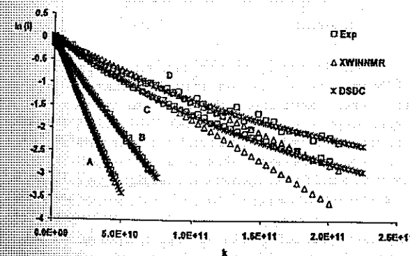
Figure 6. Plots of \ln I versus k showing the fits to experimental data using the two fitting procedures described in the text: A, fraction R, galactofuranan; B, fraction P, an arabinogalactan; C, fraction U, an arabinogalactan; D, fraction L, an arabinogalactan.
