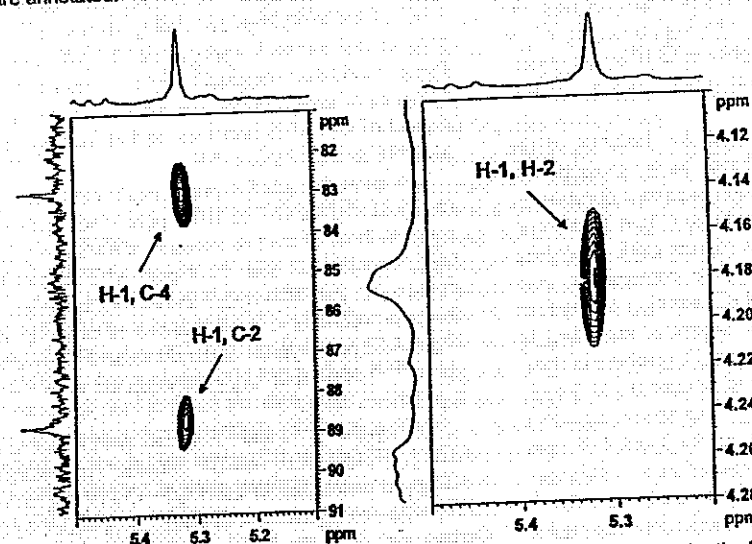
Figure 4. Portions of 500.1 MHz spectra of fraction R: on the left, the ^1\text{H} , ^{13}\text{C} HMQC spectrum; on the right, the ^1\text{H} , ^1\text{H} NOESY spectrum. The relevant correlations are annotated.
