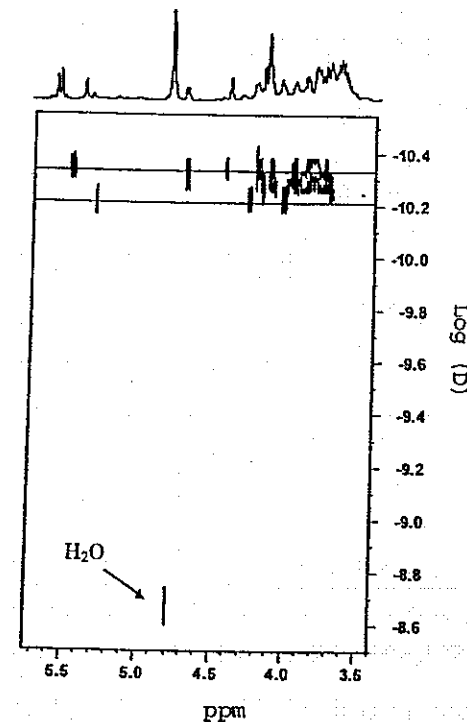
Figure 8. 500.1 MHz 1 H DOSY spectra of fraction X recorded at 14.57 mg/mL.
