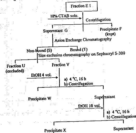
Chart 2. Flowchart Describing the Process to Obtain Fraction X Starting from Fraction E1, the Sephadex G-100 Excluded Fraction 2
