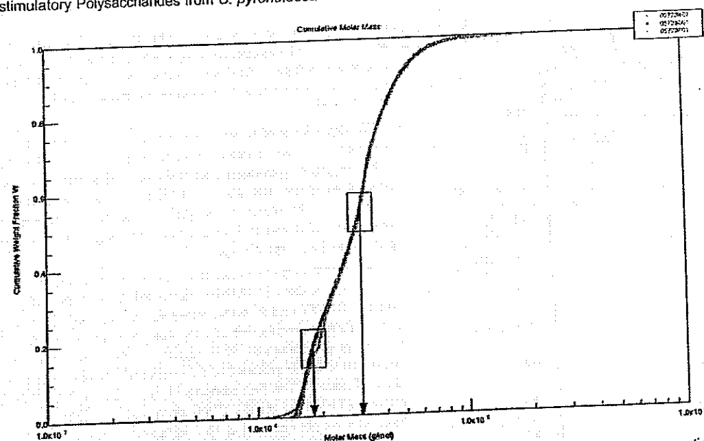
Figure 9. Cumulative molecular weight curve from SEC-MALS of fraction X. The center of the two distinct regions representing the weight average molecular weights is highlighted.
