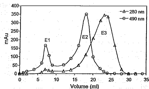
Figure 2. Size exclusion chromatography of fraction E on Sephadex G-100.
