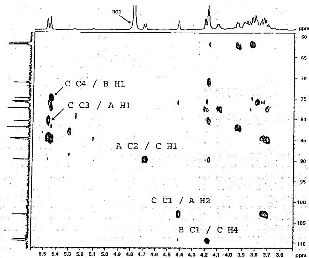
Figure 3. 500.1 MHz 1 H, 13 C HMBC spectrum of fraction I. Correlations involving glycosidic linkages are annotated.
