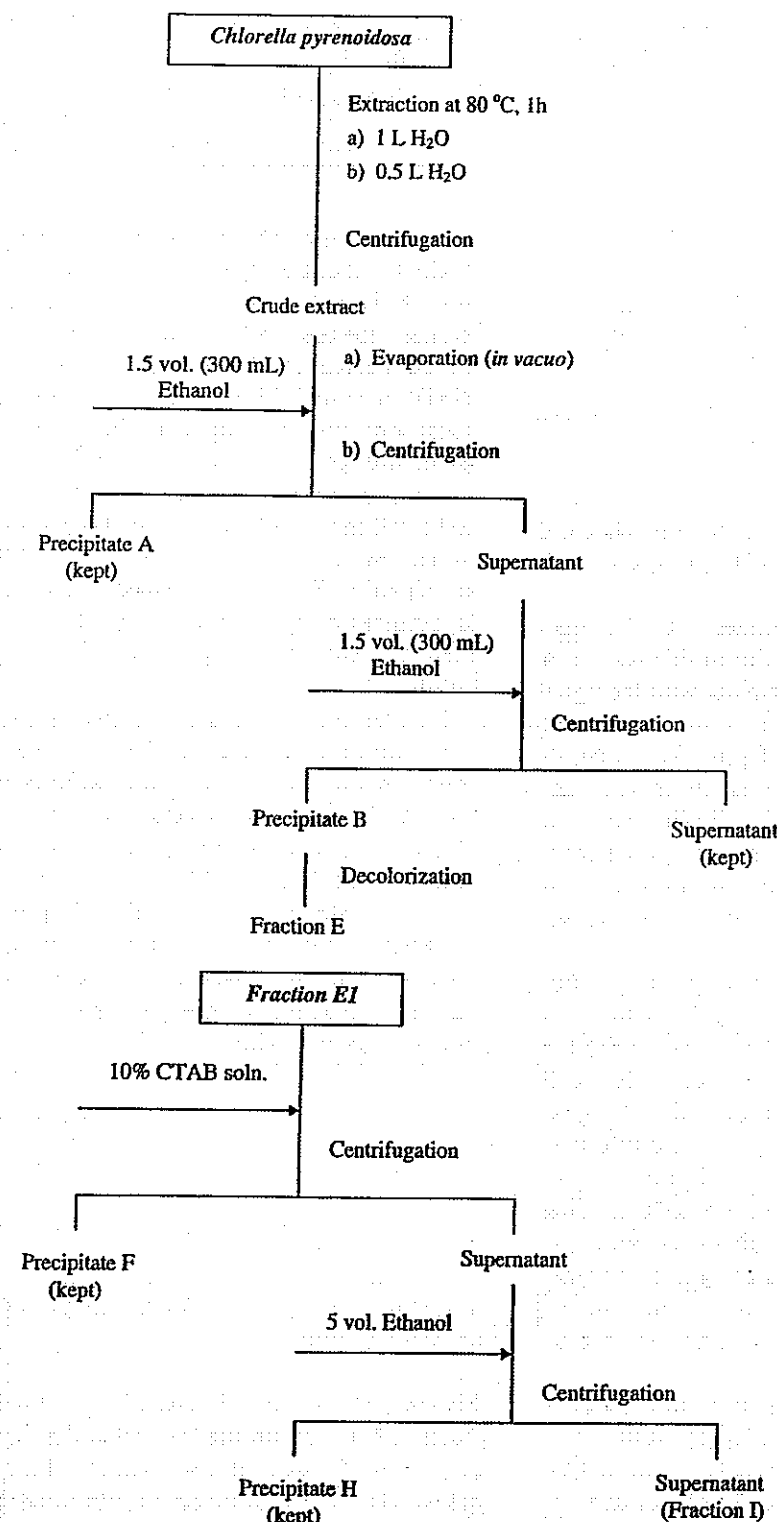
Fig. 1. Description of the process used to obtain fraction I. Part 1: isolation of E. Part 2: fractionation of E1.
