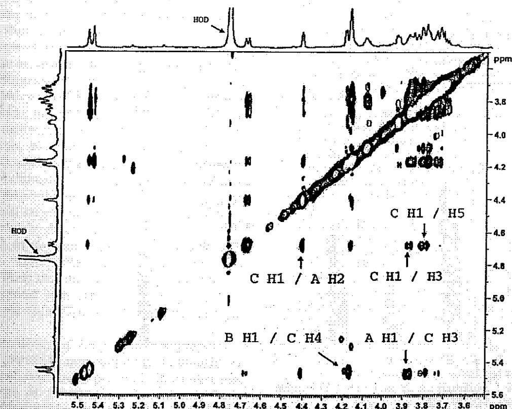
Figure 4. 500.1 MHz 1 H, 1 H NOESY spectrum of fraction I with the more relevant correlations annotated.
